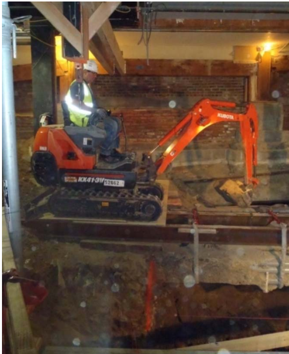
Digging the Elevator Pit: Economy Market Theater
