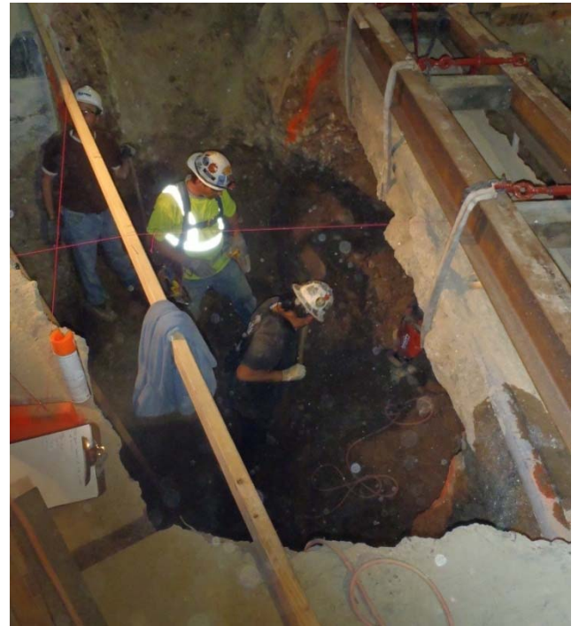
Elevator Pit: Economy Market
