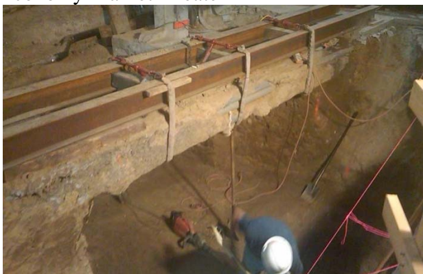
Duct Bank Shoring: Economy Market Theater
