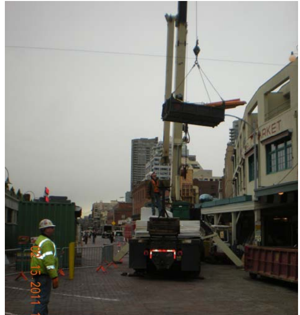
Corner Market Roof Crane Pick
